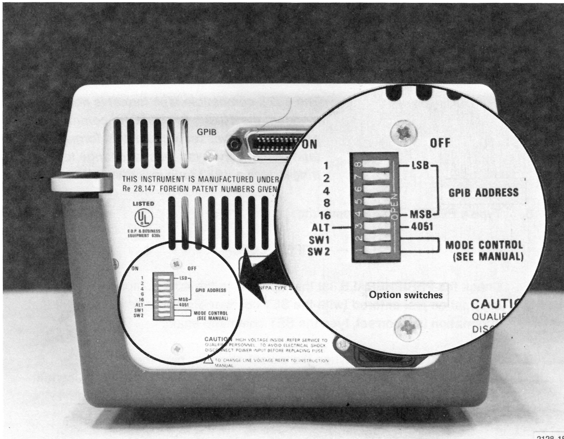
Figure 8-7. 4924 rear panel switches.
