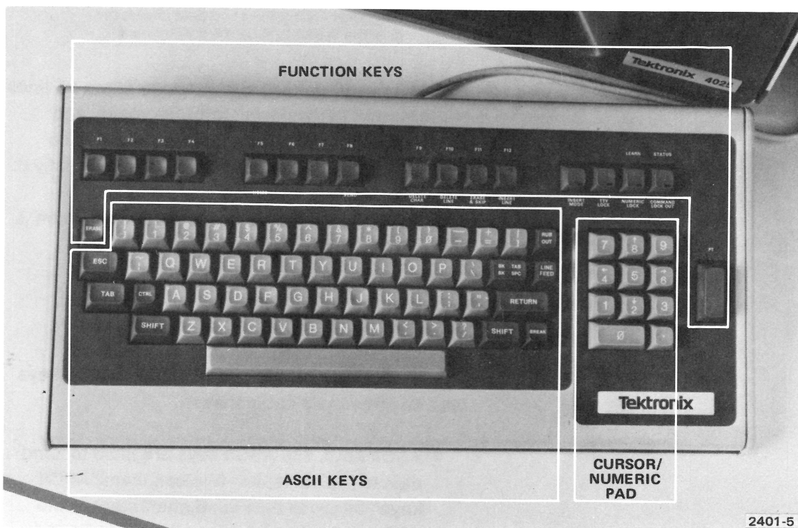
Fig. 2-2. Keyboard.
