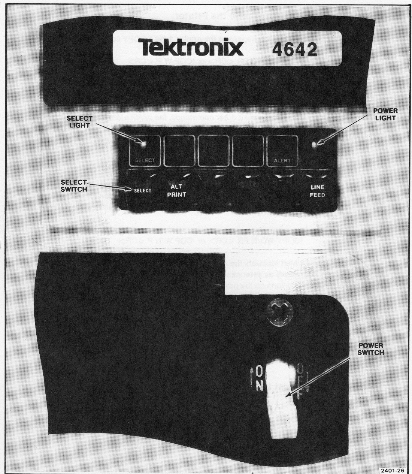
Figure 8-2. Switch settings on 4642 Printer.
