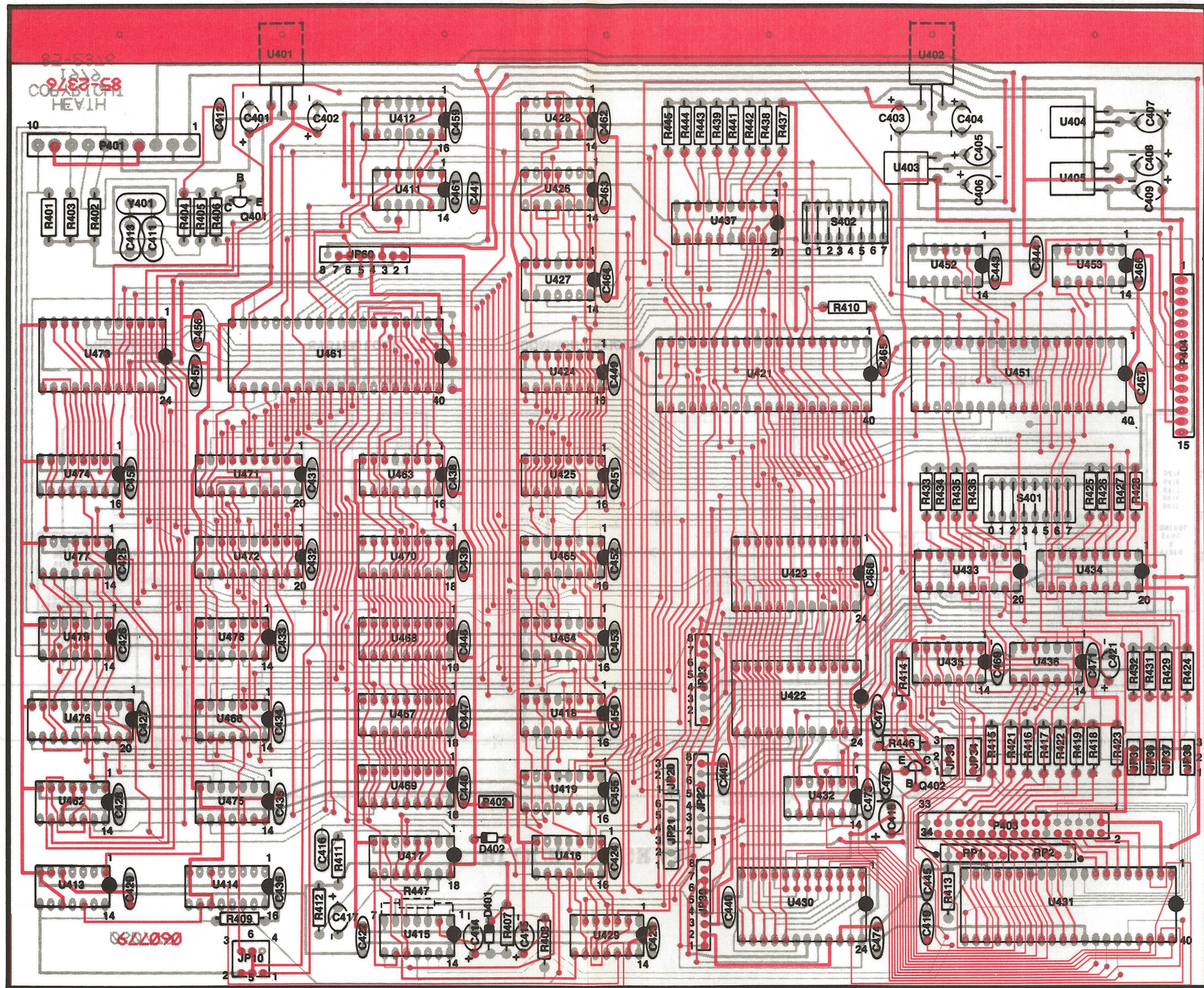
TERMINAL LOGIC CIRCUIT BOARD (Viewed from the component side) (Bottom side foil in red)
