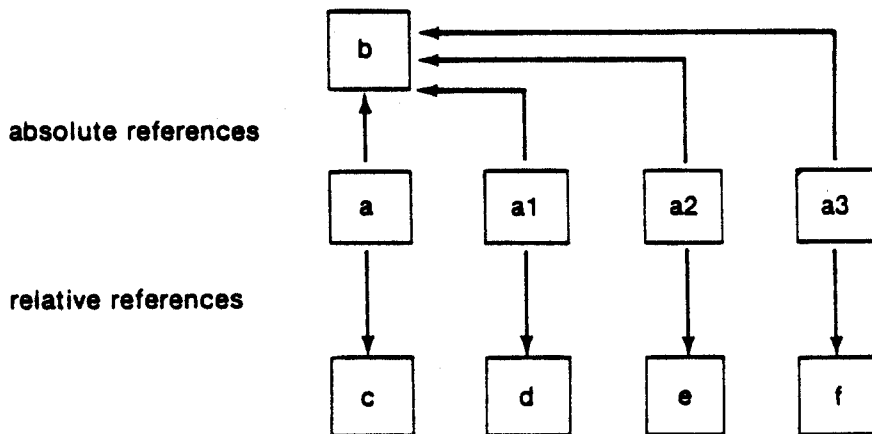
Figure 8.3. Comparison of Absolute and Relative References
