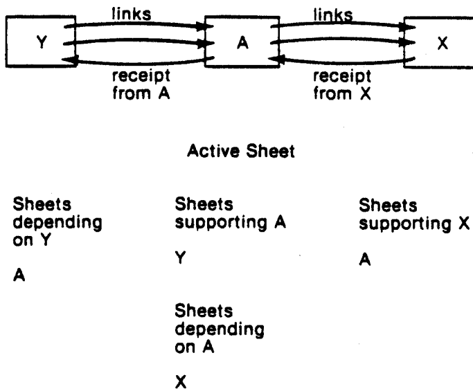
Figure 8.12. External Relationships between Worksheets
