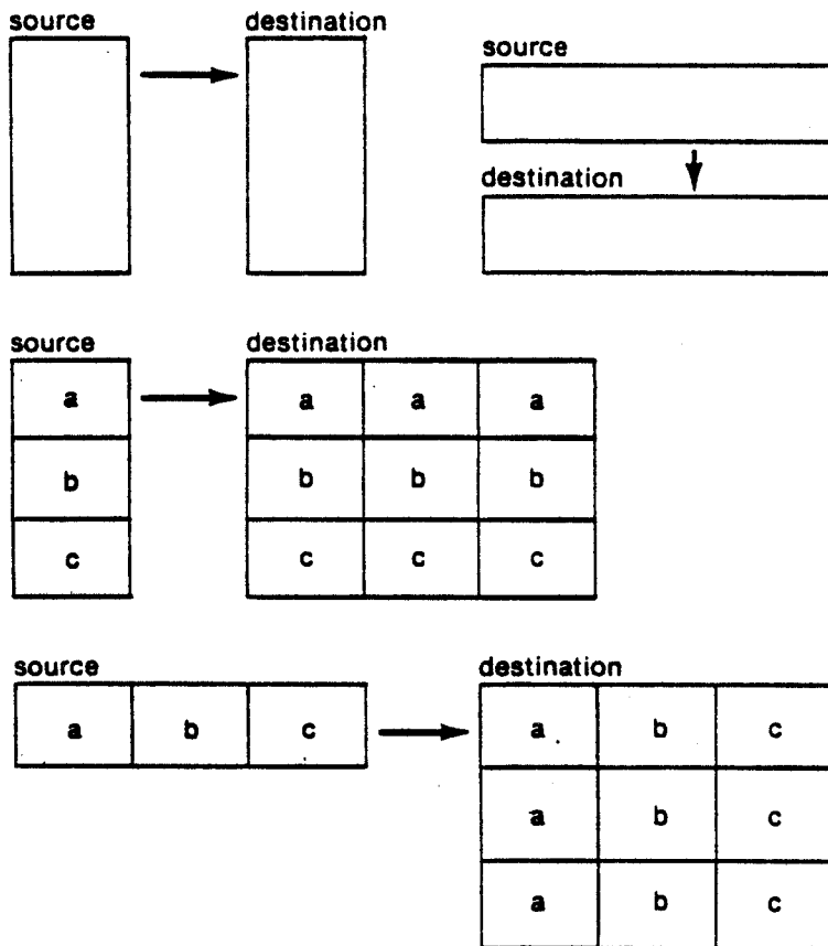
Figure 9.1. Results of Copying Vectors
